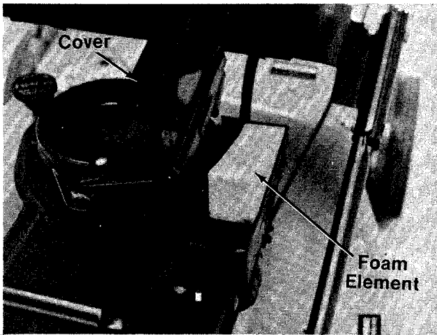
FIGURE 28. SPARK PLUG
